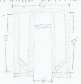
FRONT WALL FRAMING DETAIL
