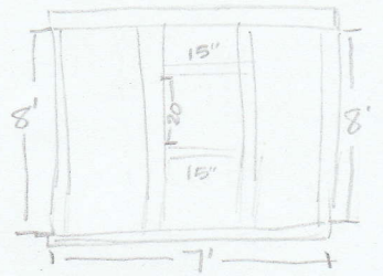
FRONT WALL FRAMING DETAIL
